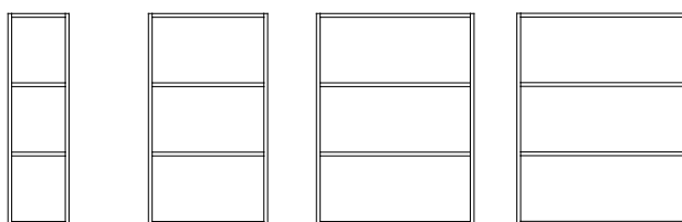
VH30/3 310x1075x370 VH60/3 605x1075x370 VH80/3 800x1075x370 VH90/3 900x1075x370
