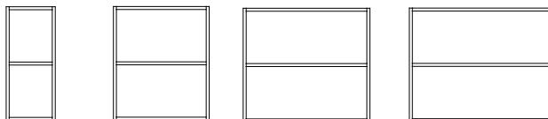
VH30/2 310x723x370 VH60/2 605x723x370 VH80/2 800x723x370 VH90/2 900x723x370
