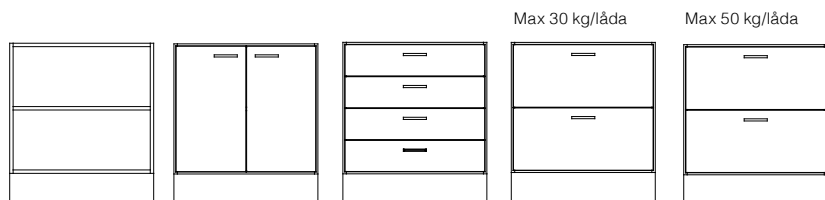
DÖ80 800x880x570 DS80 800x880x570 DL80/4L 800x880x570 DL80/2L-30 800x880x570 DL80/2L-50 800x880x570
