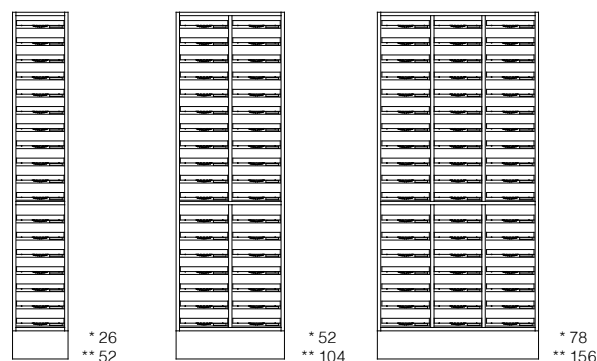
PF 18 310x1936x370
