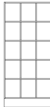
KBH90/5 900x1936x370
