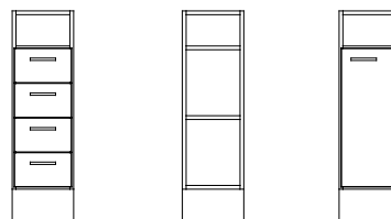
HDL30/4L 310x1057x570 HDÖ30 310x1057x570 HDS30 310x1057x570
