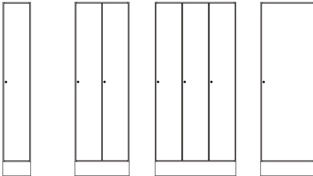
KLE30 310x1936x570 KLD60 605x1936x570 KLT90 900x1936x570 KLE60 605x1936x370
