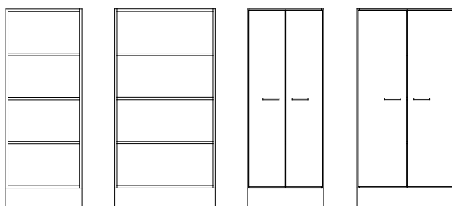
KHD60/4 605x1584x570 KHD80/4 800x1584x570 KSD60/4 605x1584x570 KSD80/4 800x1584x570
