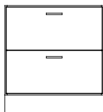
DL80/2L-30 800x880x570
