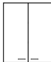
VS90/3 900x1075x370
