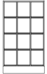
EXPO 90/12 900x1584x370
