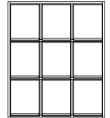
EXPO 90/9 900x1075x370
