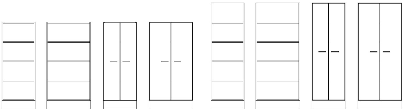
KH60/4 605x1584x370
