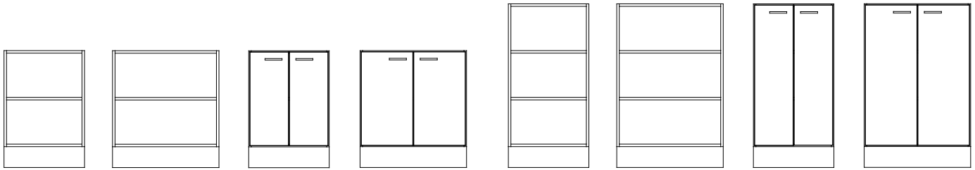
KH60/2 605x880x370
