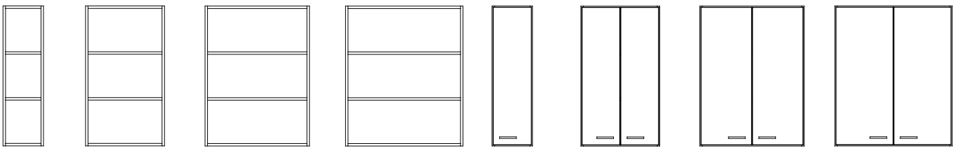
VH30/3 310x1075x370 VH60/3 605x1075x370 VH80/3 800x1075x370 VH90/3 900x1075x370 VS30/3 310x1075x370 VS60/3 605x1075x370 VS80/3 800x1075x370 VS90/3 900x1075x370
