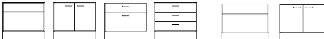
SDÖ80 800x704x570 SDS80 800x704x570 SD80/2L 100% 800x704x570 SD80/3L 100% 800x704x570 SDÖ90 900x704x570 SDS90 900x704x570
