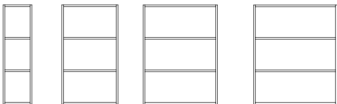
VH30/3 310x1075x370 VH60/3 605x1075x370
